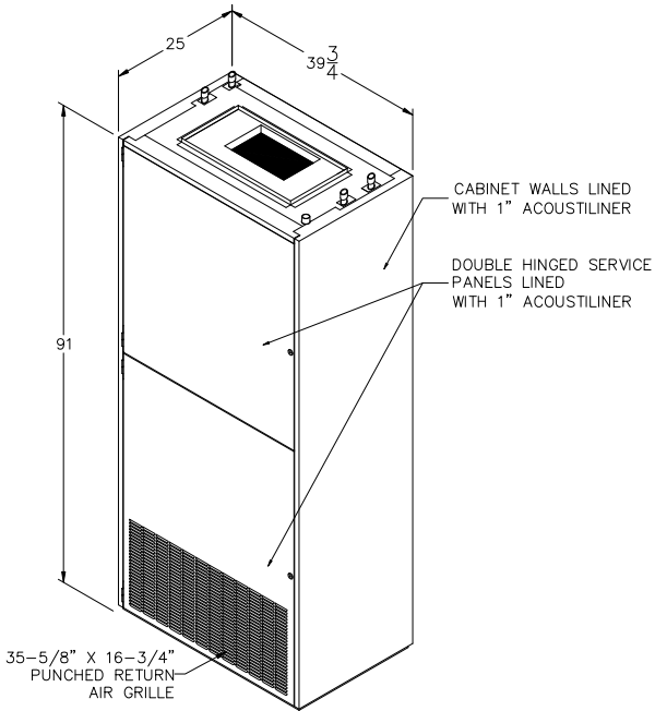
ISOMETRIC VIEW
