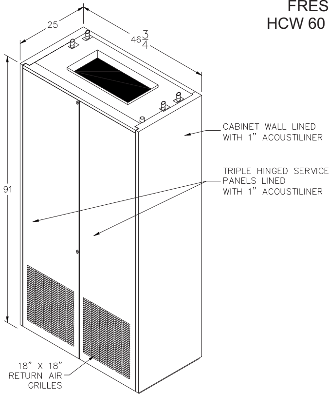
ISOMETRIC VIEW
