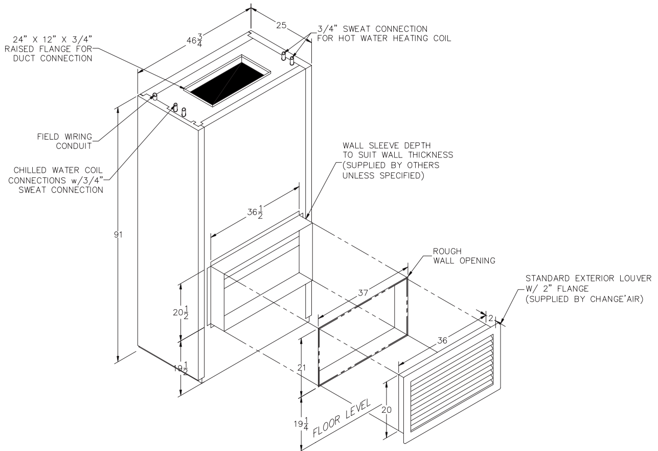
INSTALLATION VIEW
